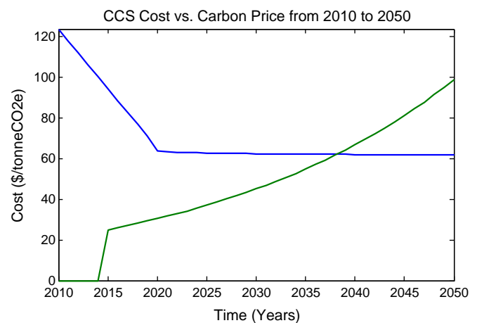
Fig. 1. CCS deployment "price gap." The green line is a carbon price scenario, and the blue line an estimate of CCS costs. (For interpretation of the references to colour in this figure legend, the reader is referred to the web version of this article.)
