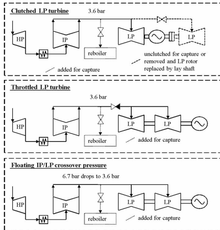
Figure 1 Potential Steam Turbine Modifications for Integrated Retrofits
